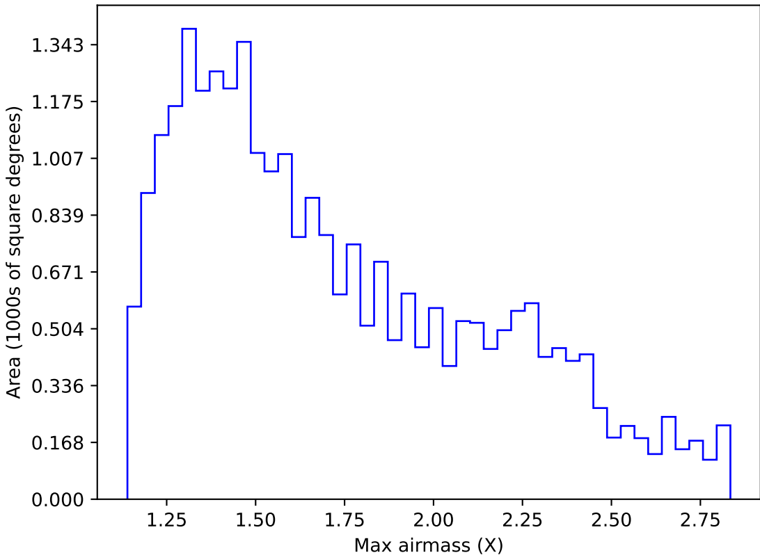
too_elab_r8_d2_gz_v3.4_10yrs Yr 1 i band: Max airmass
