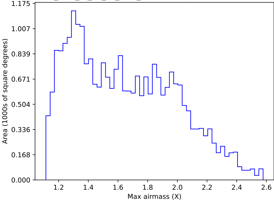
too_elab_r8_d2_gz_v3.4_10yrs Yr 1 g band: Max airmass
