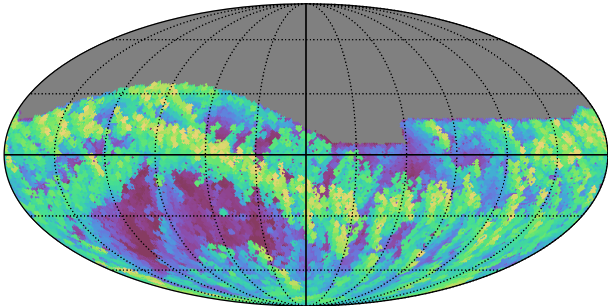
too_elab_r8_d2_gz_v3.4_10yrs Yr 1 all bands: Max airmass
