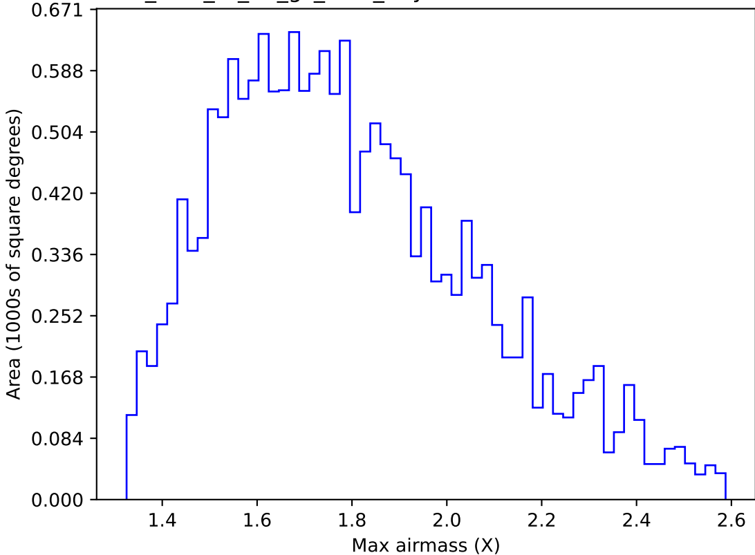
too_elab_r8_d2_gz_v3.4_10yrs WFD u band: Max airmass
