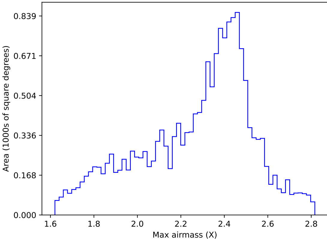
too_elab_r8_d2_gz_v3.4_10yrs WFD r band: Max airmass
