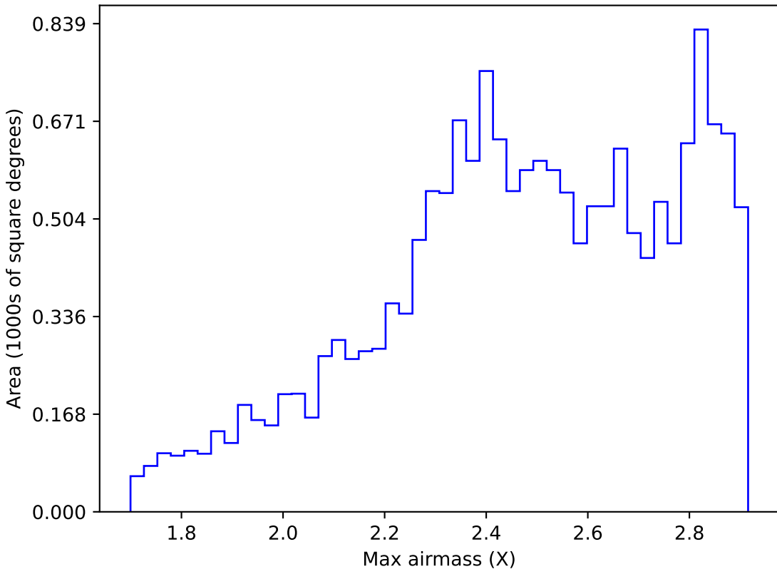
too_elab_r8_d2_gz_v3.4_10yrs WFD i band: Max airmass
