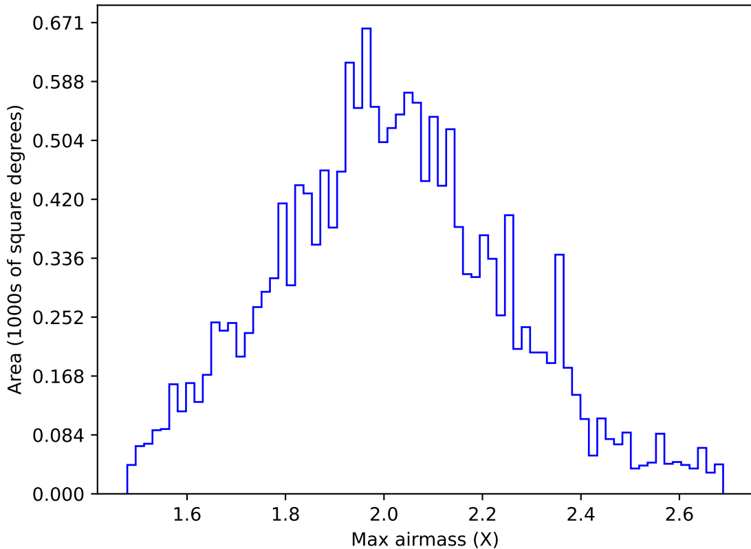
too_elab_r8_d2_gz_v3.4_10yrs WFD g band: Max airmass
