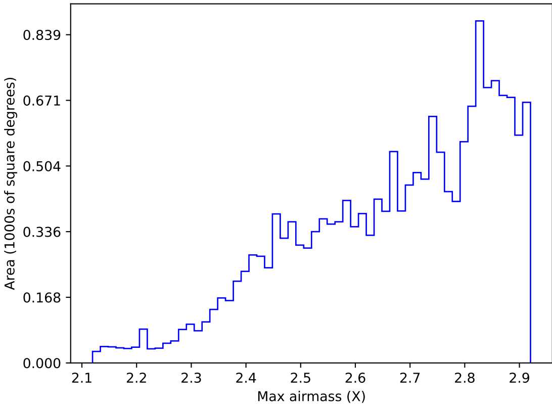
too_elab_r8_d2_gz_v3.4_10yrs WFD all bands: Max airmass
