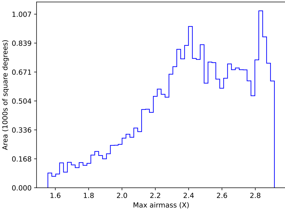
too_elab_r8_d2_gz_v3.4_10yrs All sky z band: Max airmass
