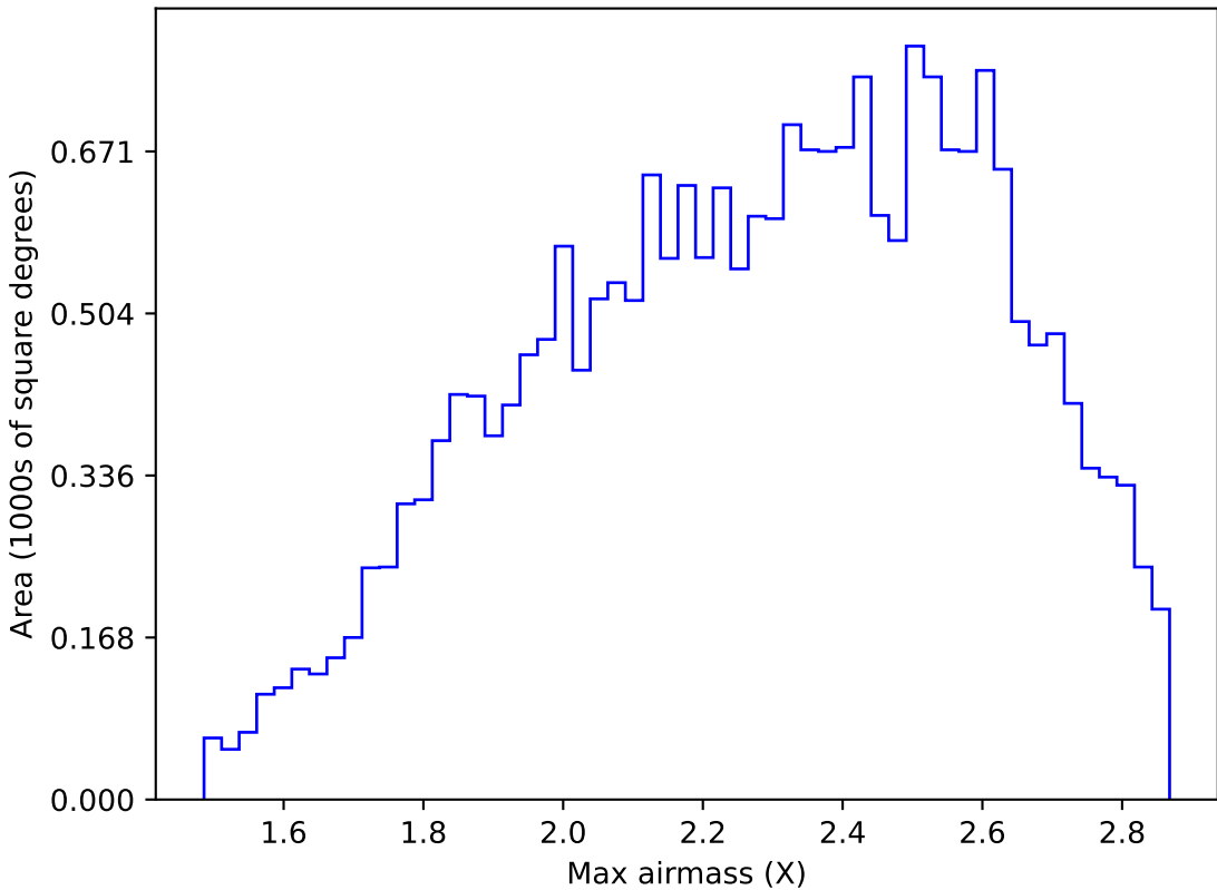
too_elab_r8_d2_gz_v3.4_10yrs All sky y band: Max airmass
