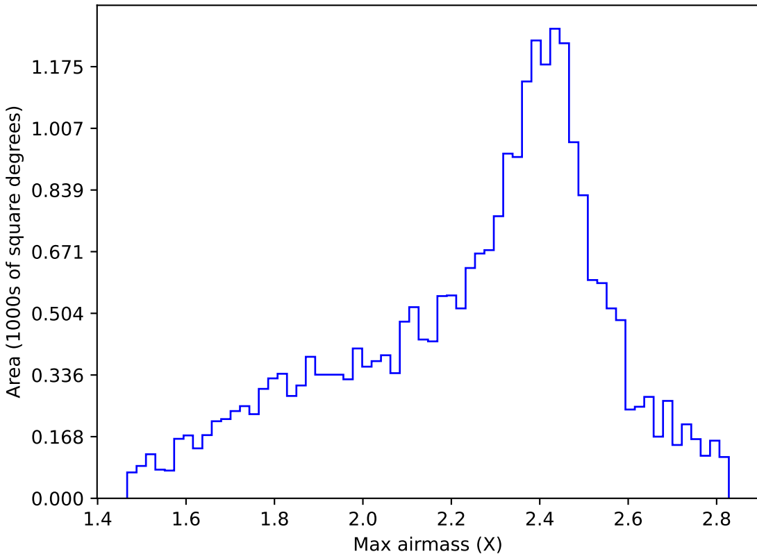
too_elab_r8_d2_gz_v3.4_10yrs All sky r band: Max airmass
