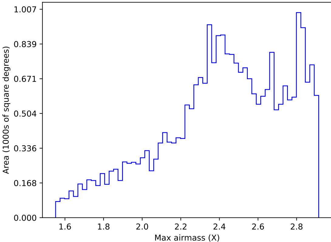
too_elab_r8_d2_gz_v3.4_10yrs All sky i band: Max airmass
