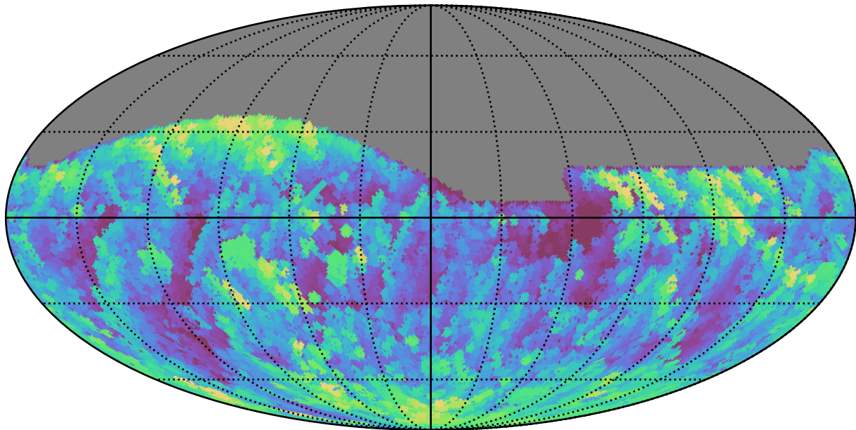
too_elab_r8_d2_gz_v3.4_10yrs All sky g band: Max airmass
