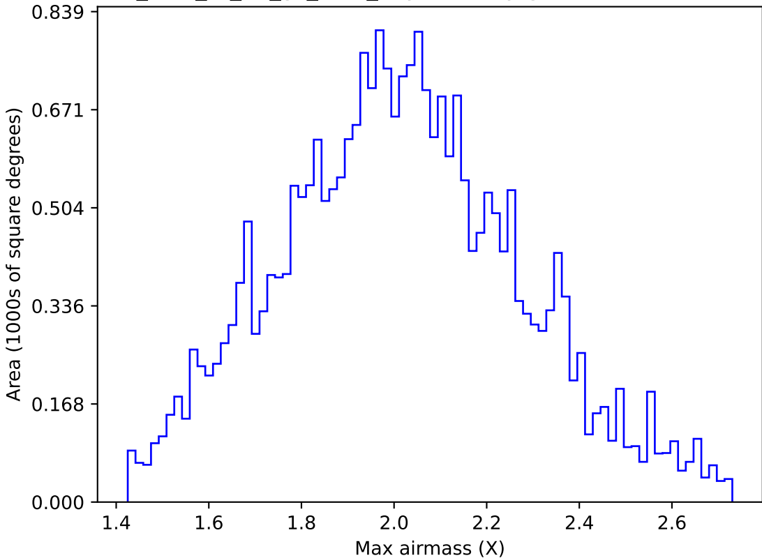
too_elab_r8_d2_gz_v3.4_10yrs All sky g band: Max airmass
