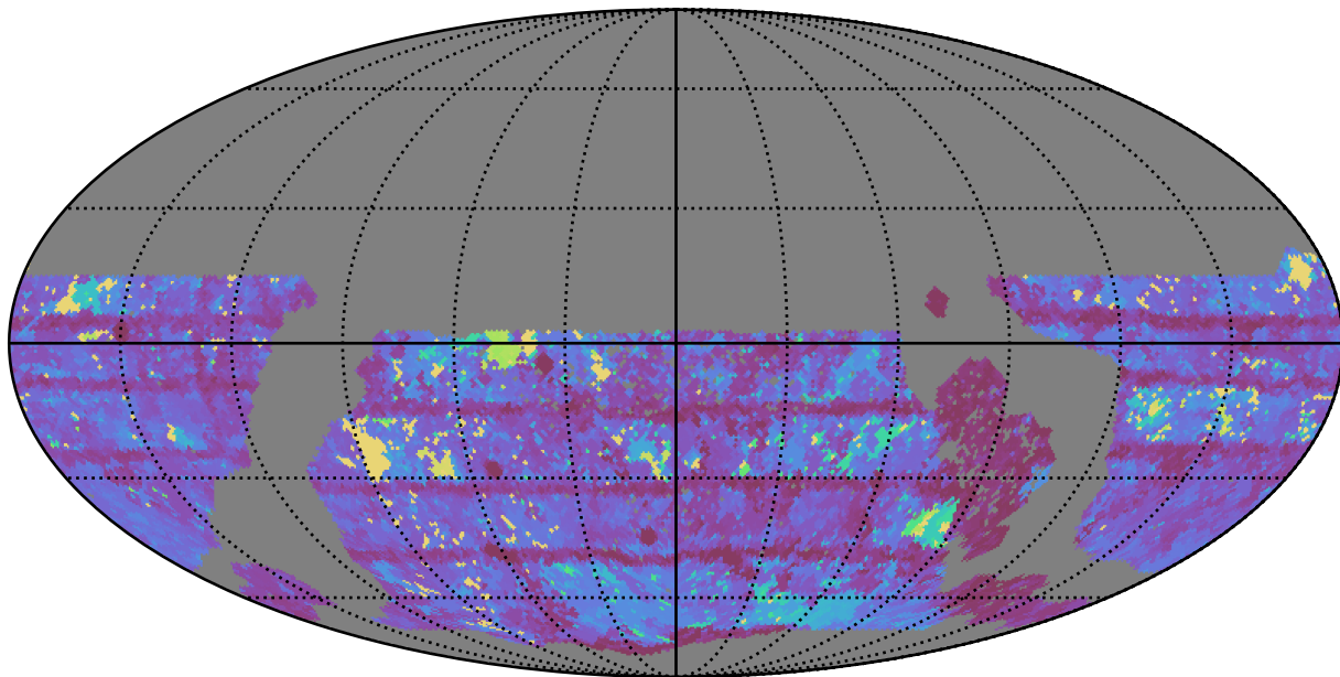
too_elab_r8_d2_gz_v3.4_10yrs WFD z band: Max Inter-Night Gap
