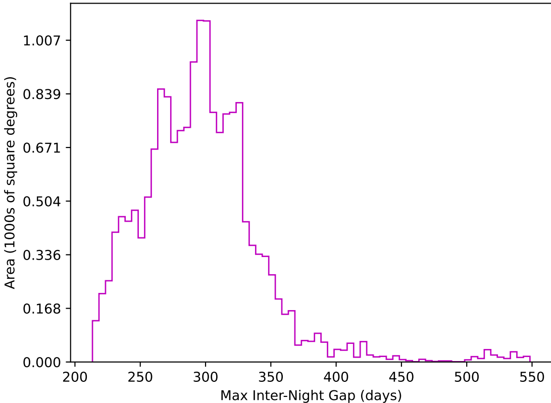
too_elab_r8_d2_gz_v3.4_10yrs WFD z band: Max Inter-Night Gap
