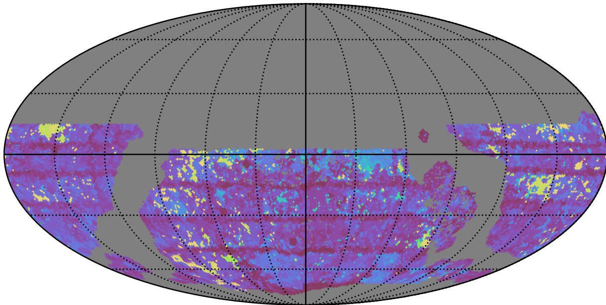
too_elab_r8_d2_gz_v3.4_10yrs WFD y band: Max Inter-Night Gap
