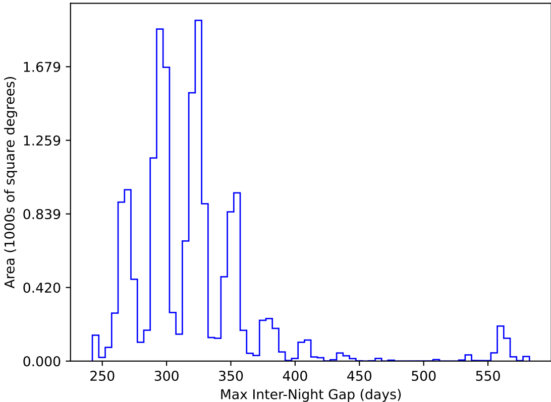
too_elab_r8_d2_gz_v3.4_10yrs WFD y band: Max Inter-Night Gap
