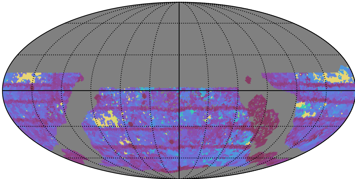
too_elab_r8_d2_gz_v3.4_10yrs WFD r band: Max Inter-Night Gap
