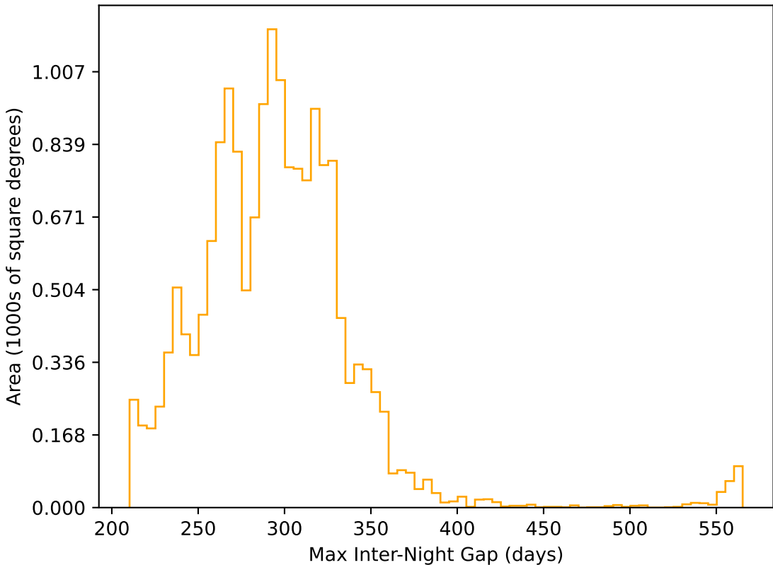
too_elab_r8_d2_gz_v3.4_10yrs WFD r band: Max Inter-Night Gap
