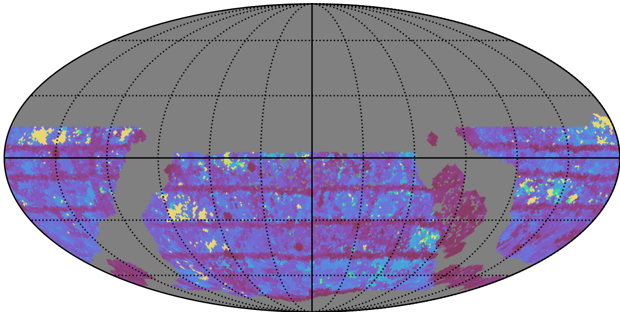
too_elab_r8_d2_gz_v3.4_10yrs WFD i band: Max Inter-Night Gap
