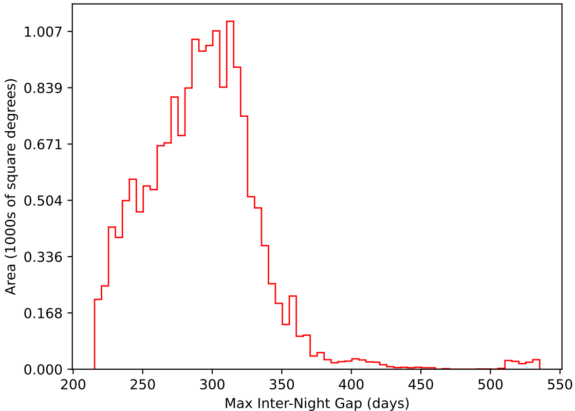
too_elab_r8_d2_gz_v3.4_10yrs WFD i band: Max Inter-Night Gap
