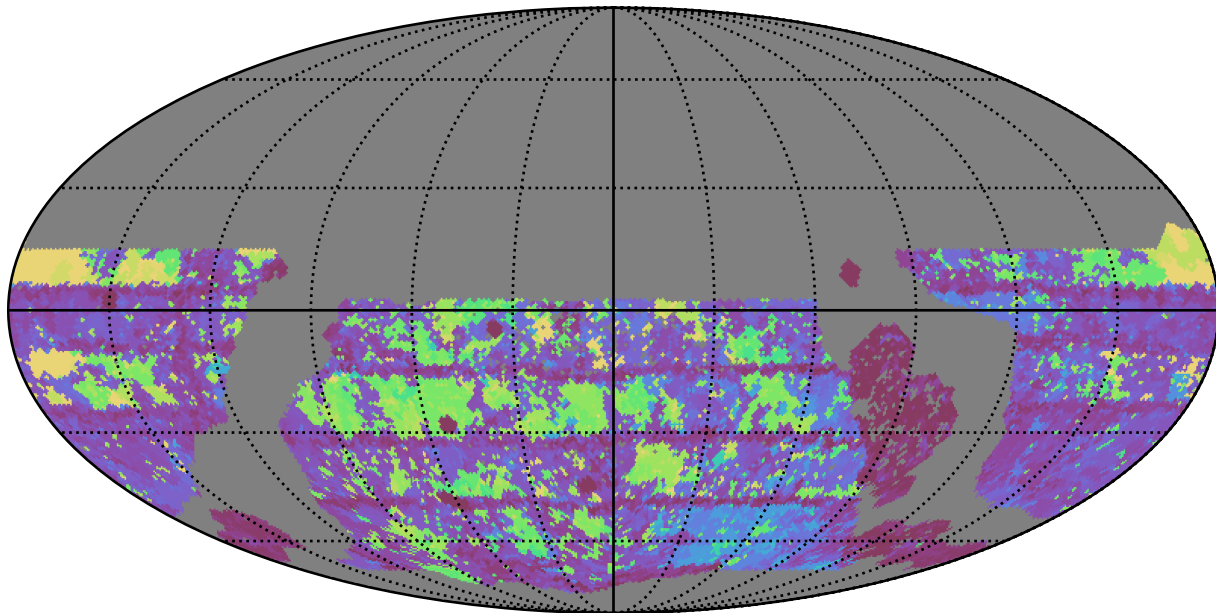
too_elab_r8_d2_gz_v3.4_10yrs WFD g band: Max Inter-Night Gap
