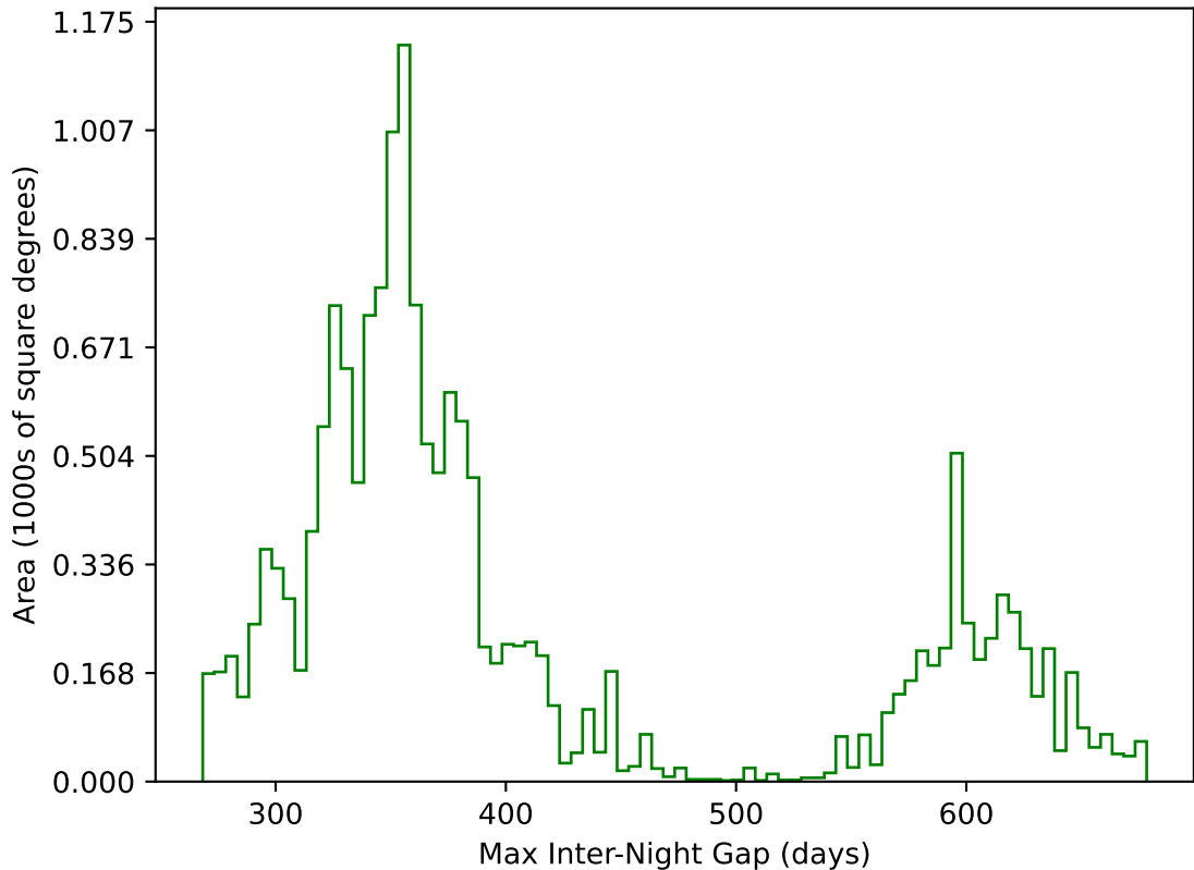
too_elab_r8_d2_gz_v3.4_10yrs WFD g band: Max Inter-Night Gap
