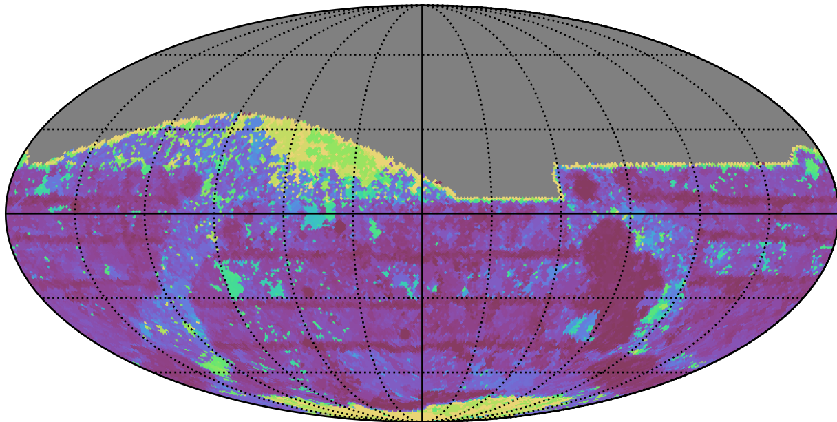
too_elab_r8_d2_gz_v3.4_10yrs All sky z band: Max Inter-Night Gap
