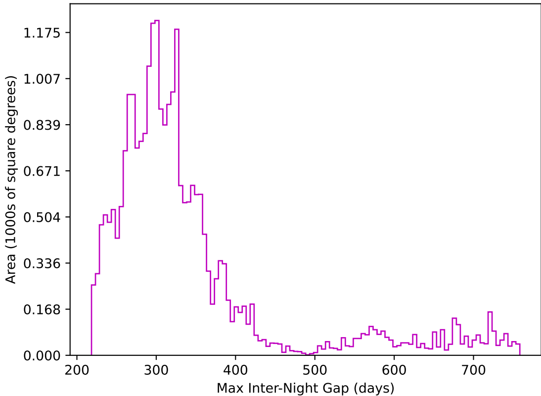
too_elab_r8_d2_gz_v3.4_10yrs All sky z band: Max Inter-Night Gap
