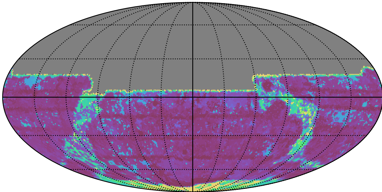
too_elab_r8_d2_gz_v3.4_10yrs All sky y band: Max Inter-Night Gap
