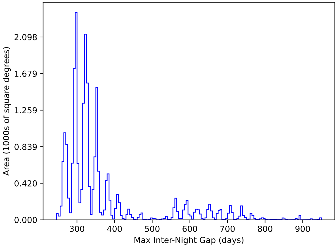
too_elab_r8_d2_gz_v3.4_10yrs All sky y band: Max Inter-Night Gap
