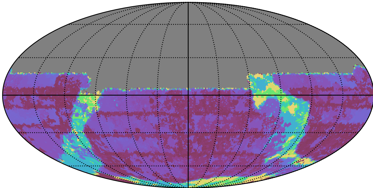
too_elab_r8_d2_gz_v3.4_10yrs All sky u band: Max Inter-Night Gap
