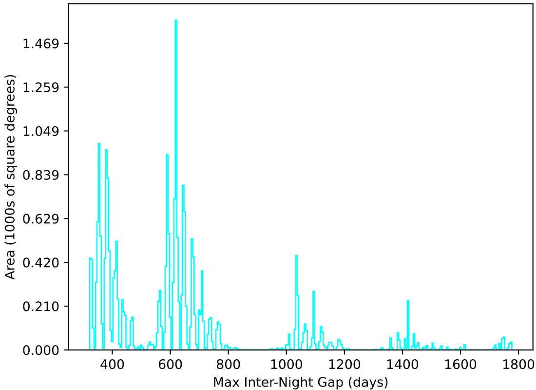
too_elab_r8_d2_gz_v3.4_10yrs All sky u band: Max Inter-Night Gap
