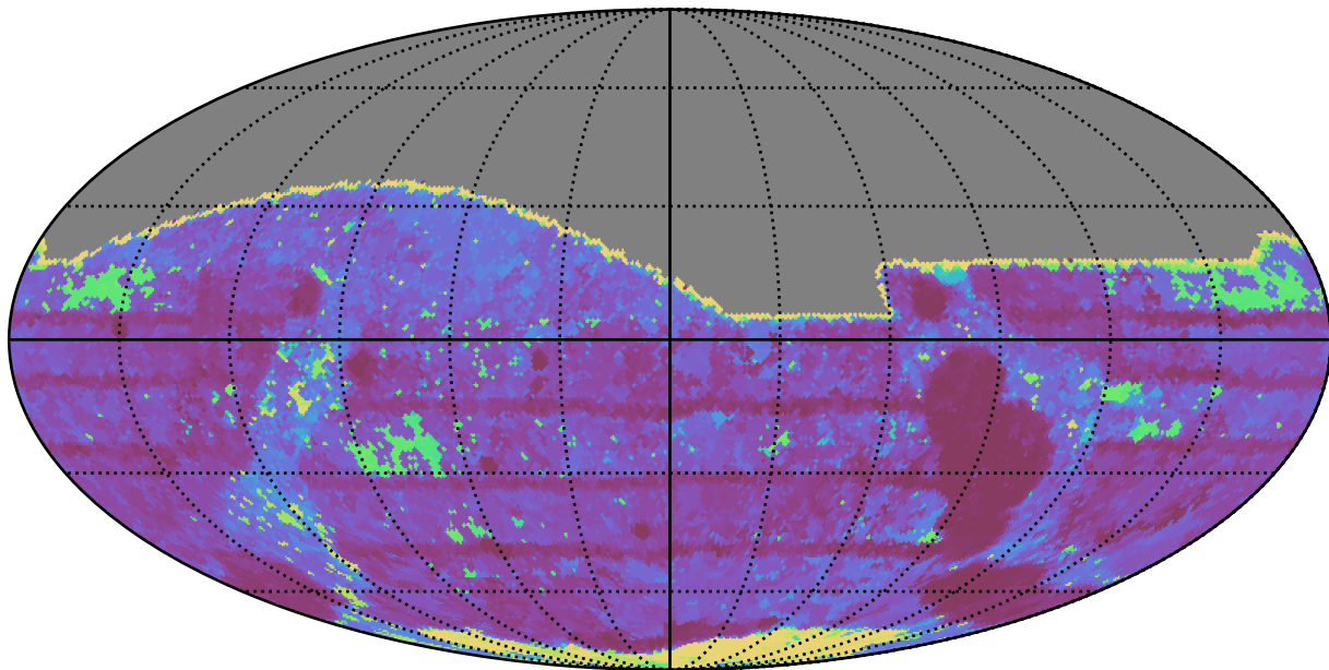
too_elab_r8_d2_gz_v3.4_10yrs All sky r band: Max Inter-Night Gap
