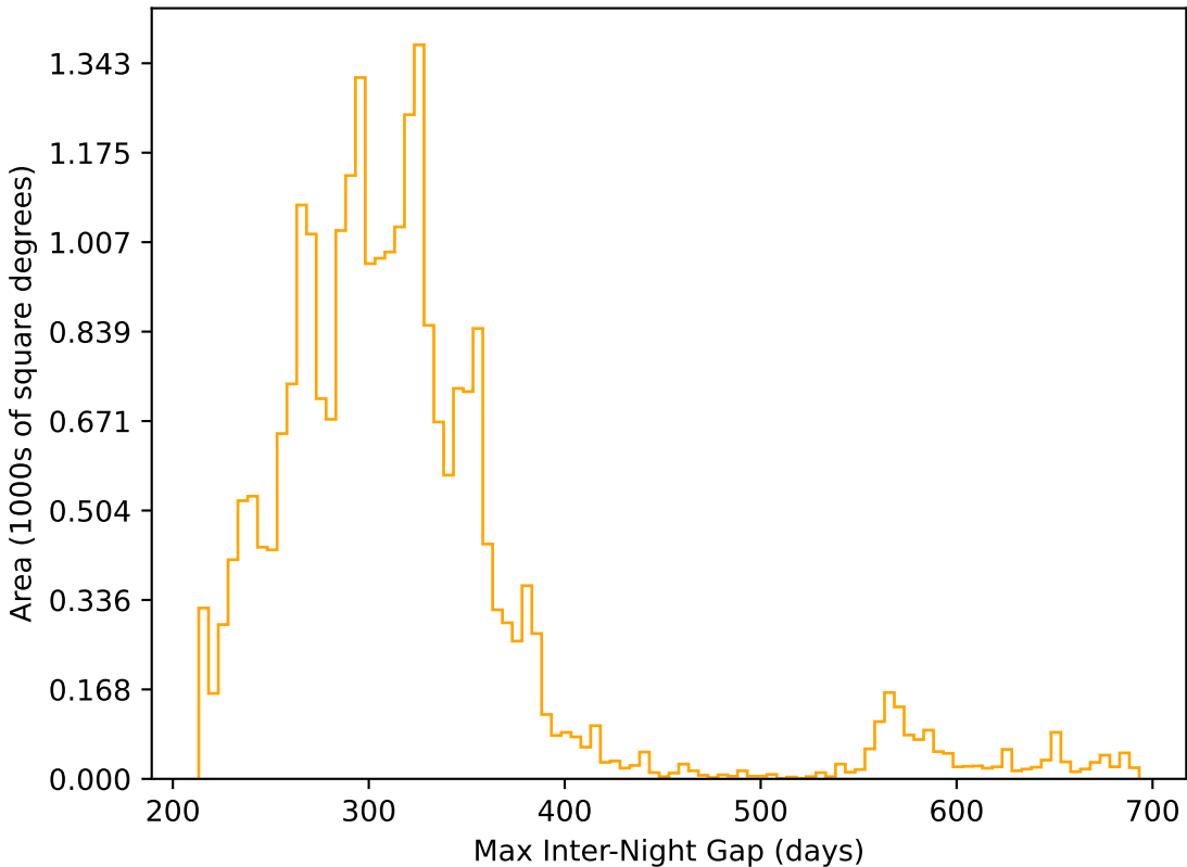
too_elab_r8_d2_gz_v3.4_10yrs All sky r band: Max Inter-Night Gap
