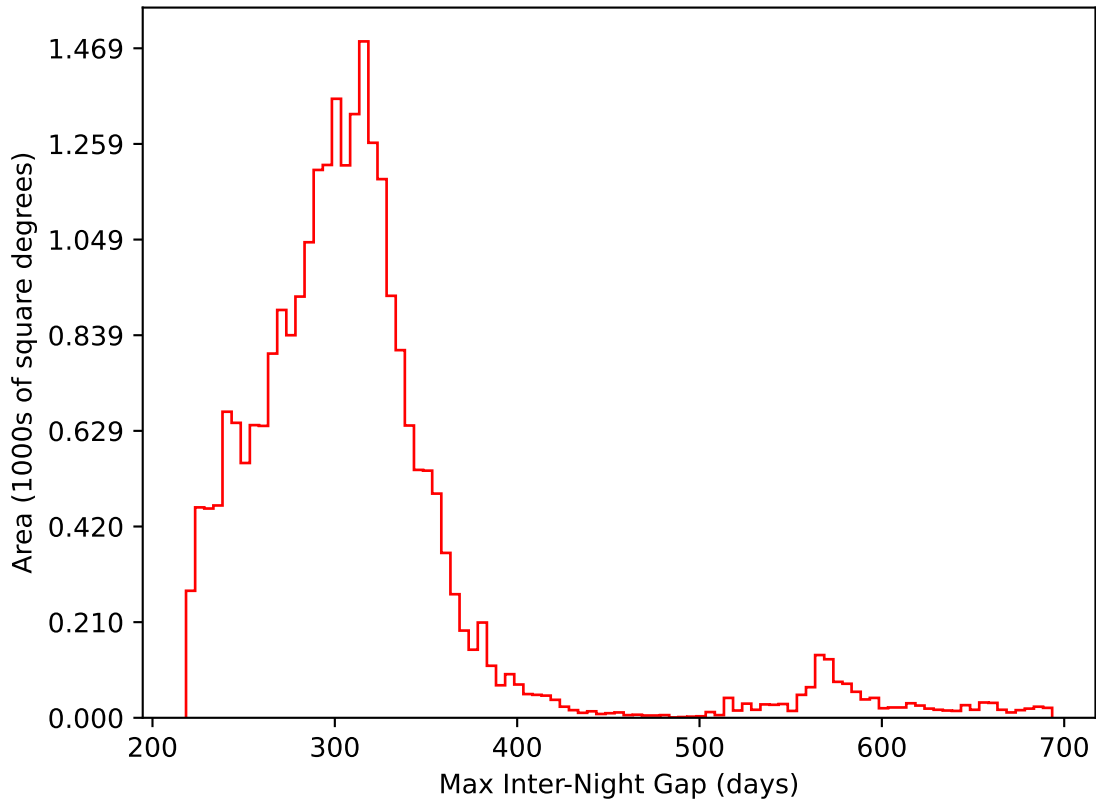
too_elab_r8_d2_gz_v3.4_10yrs All sky i band: Max Inter-Night Gap
