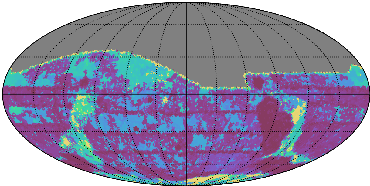
too_elab_r8_d2_gz_v3.4_10yrs All sky g band: Max Inter-Night Gap
