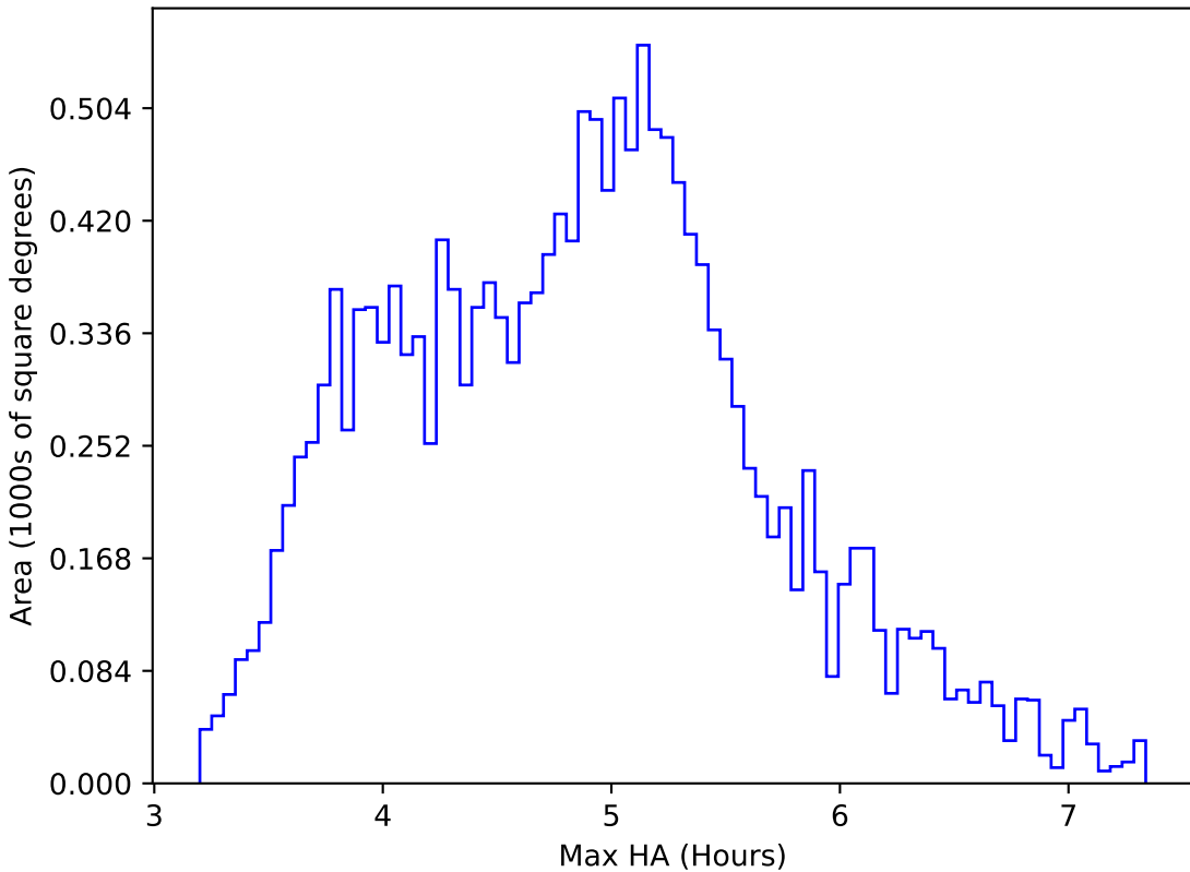
too_elab_r8_d2_gz_v3.4_10yrs WFD z band: Max HA
