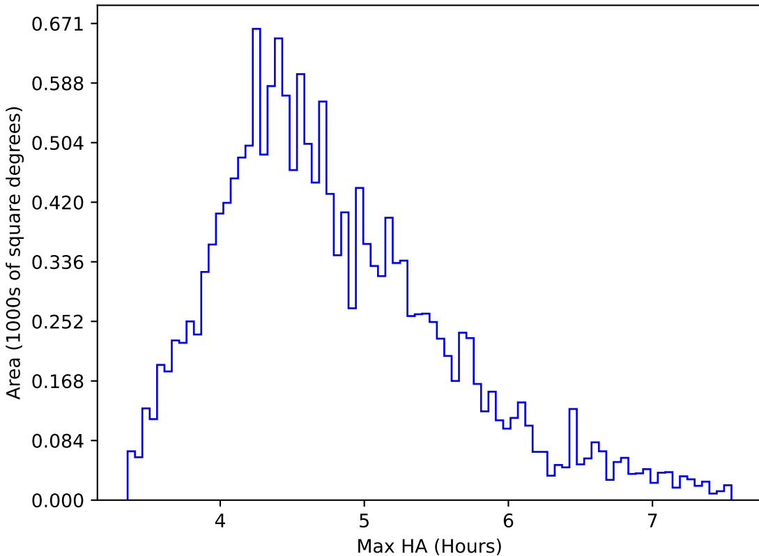
too_elab_r8_d2_gz_v3.4_10yrs WFD y band: Max HA
