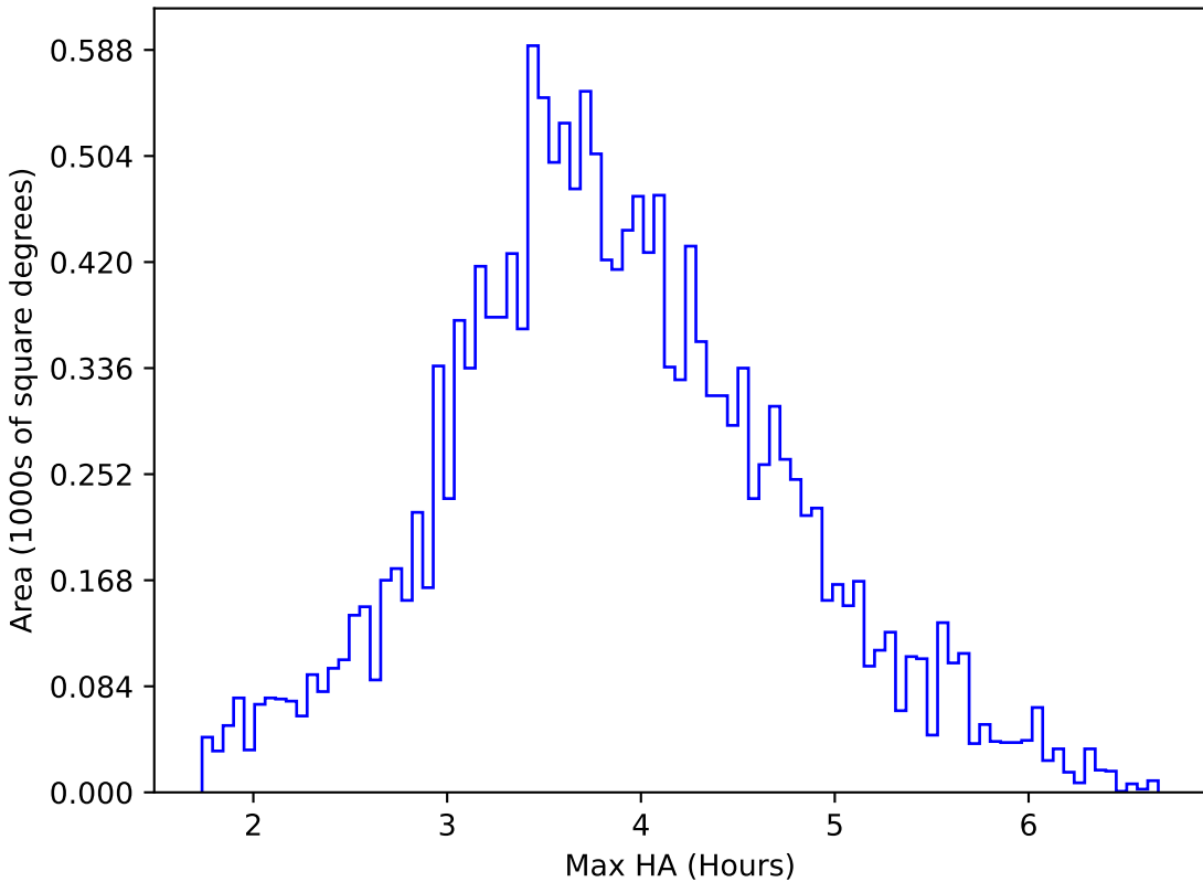
too_elab_r8_d2_gz_v3.4_10yrs WFD u band: Max HA
