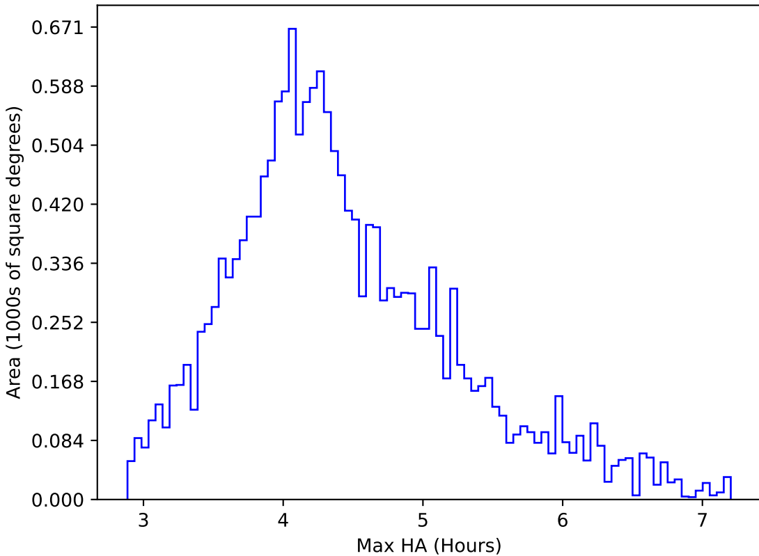
too_elab_r8_d2_gz_v3.4_10yrs WFD r band: Max HA
