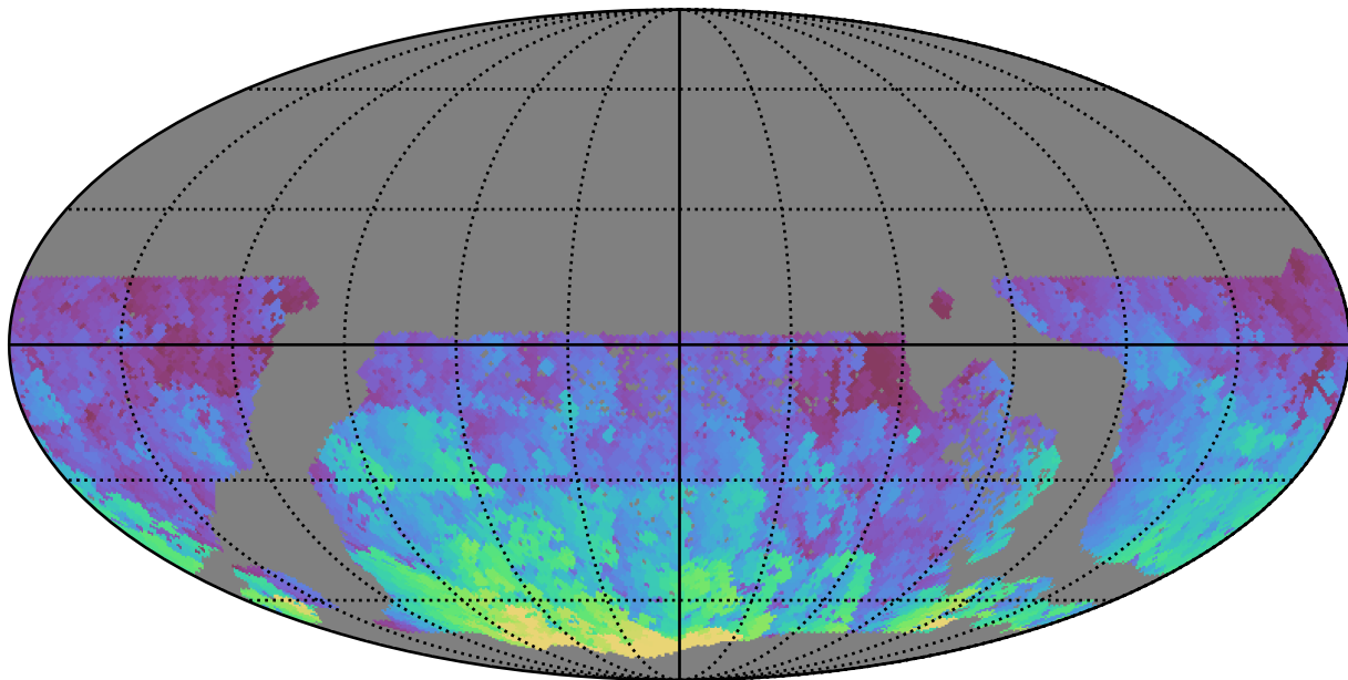
too_elab_r8_d2_gz_v3.4_10yrs WFD g band: Max HA
