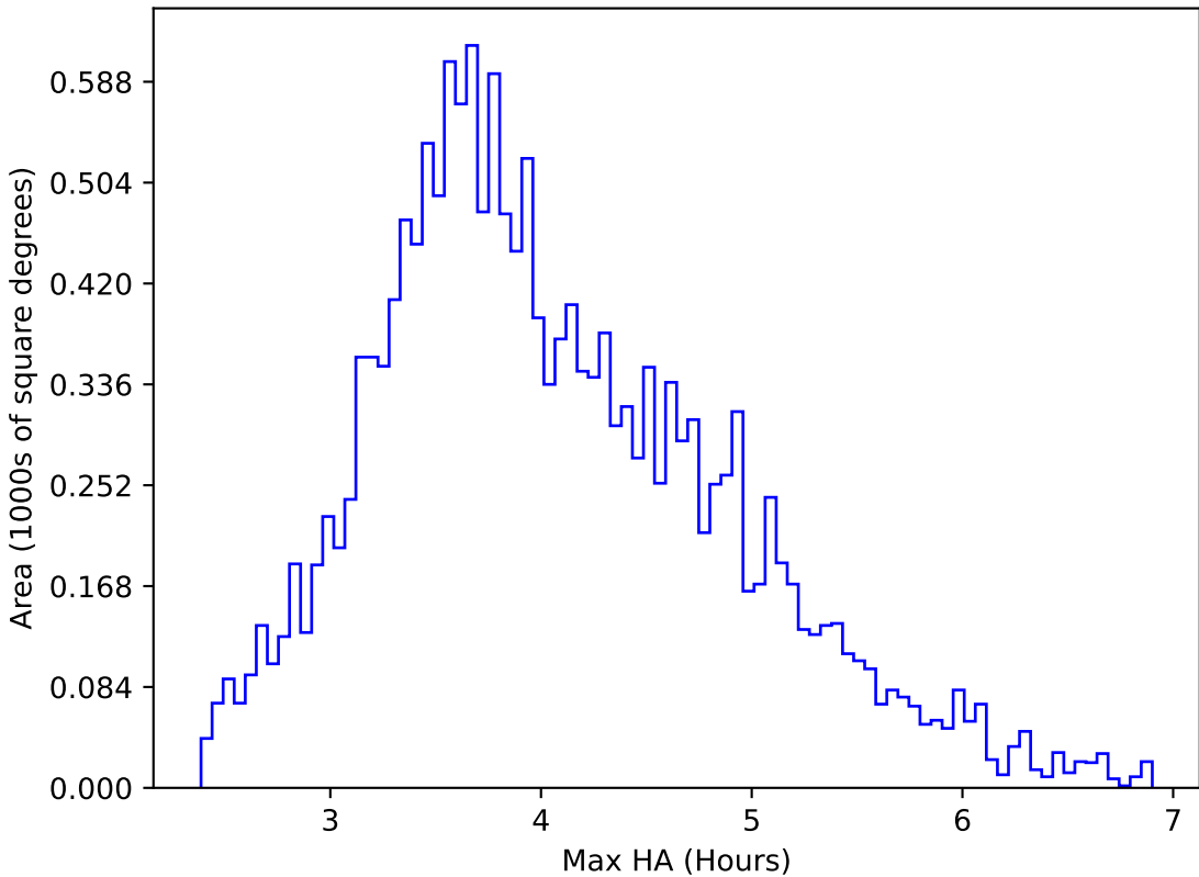
too_elab_r8_d2_gz_v3.4_10yrs WFD g band: Max HA
