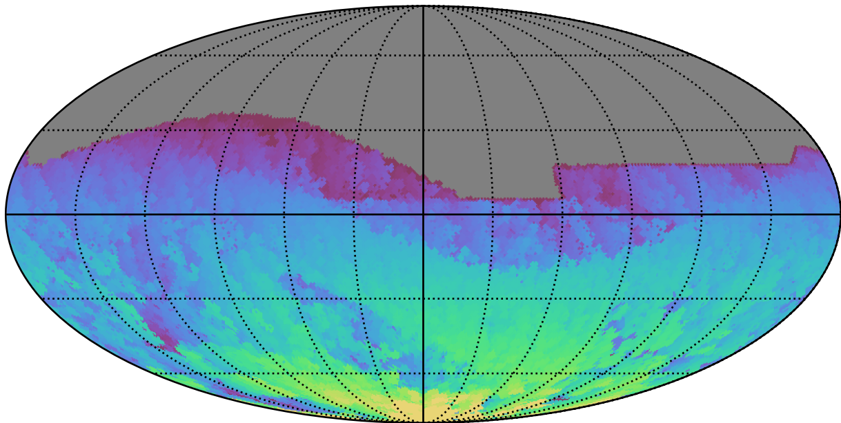
too_elab_r8_d2_gz_v3.4_10yrs All sky z band: Max HA
