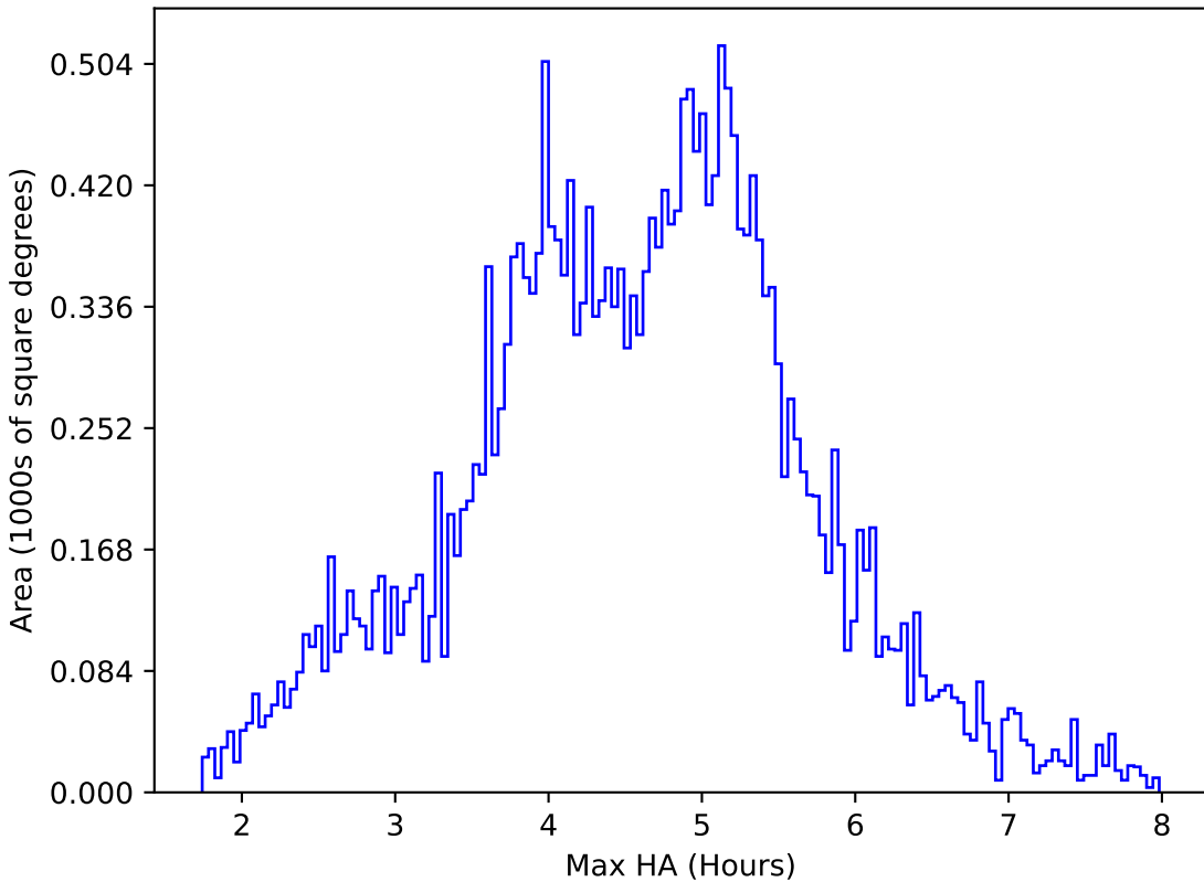
too_elab_r8_d2_gz_v3.4_10yrs All sky z band: Max HA
