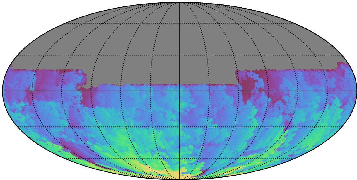
too_elab_r8_d2_gz_v3.4_10yrs All sky u band: Max HA
