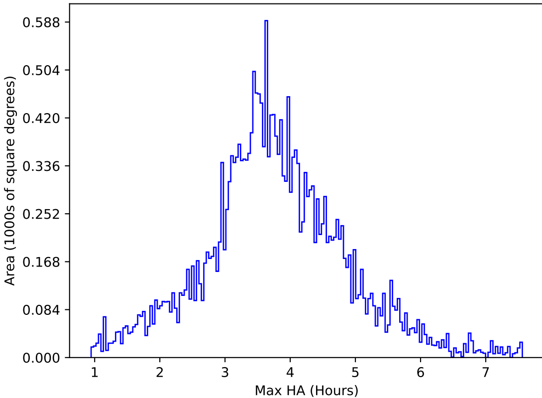
too_elab_r8_d2_gz_v3.4_10yrs All sky u band: Max HA
