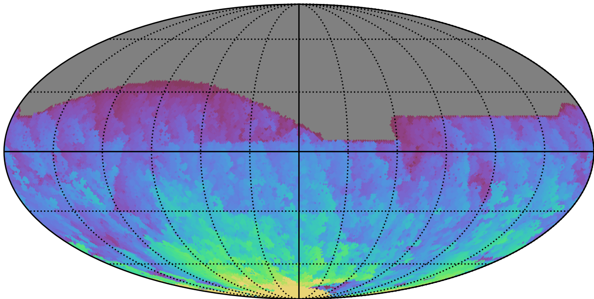
too_elab_r8_d2_gz_v3.4_10yrs All sky r band: Max HA
