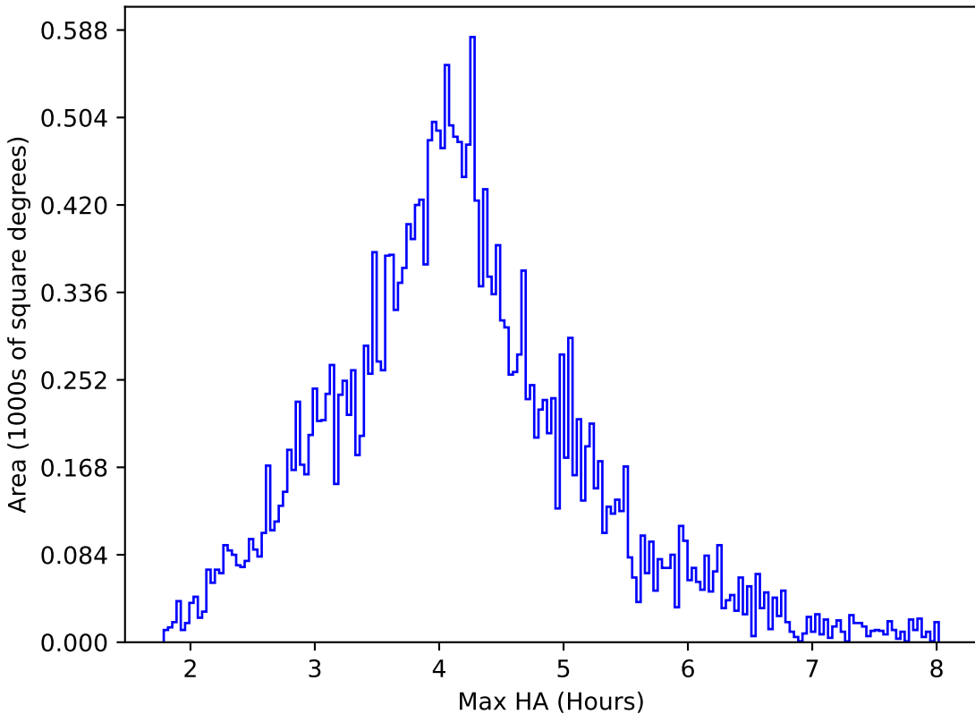
too_elab_r8_d2_gz_v3.4_10yrs All sky r band: Max HA
