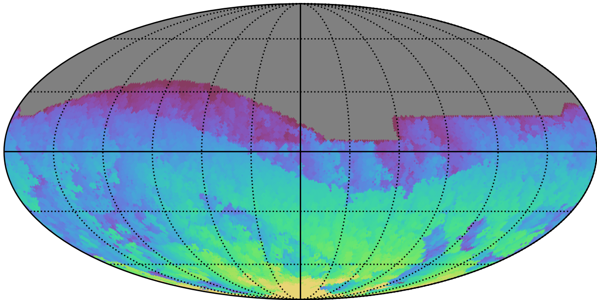
too_elab_r8_d2_gz_v3.4_10yrs All sky i band: Max HA
