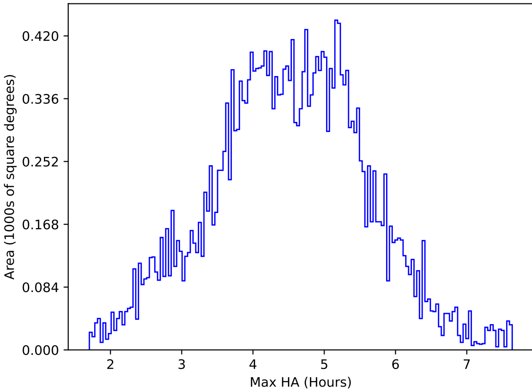
too_elab_r8_d2_gz_v3.4_10yrs All sky i band: Max HA
