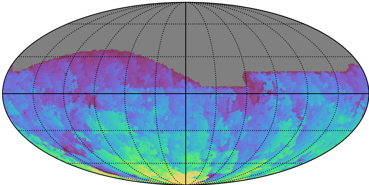
too_elab_r8_d2_gz_v3.4_10yrs All sky g band: Max HA
