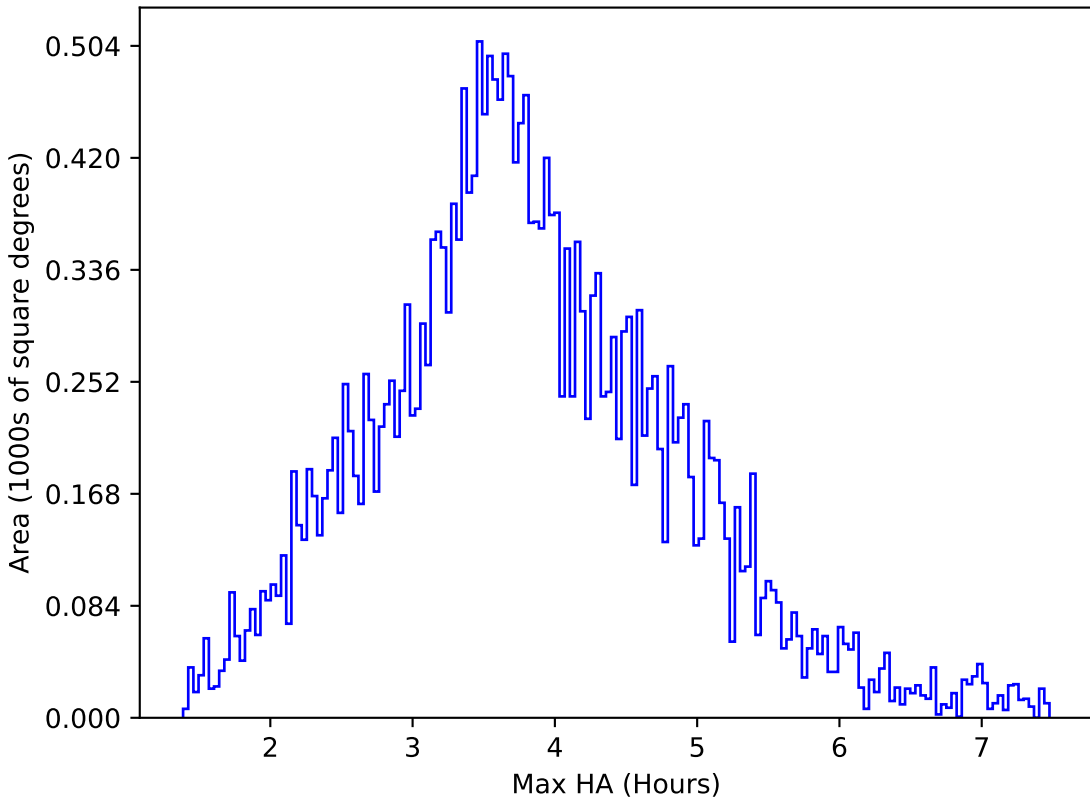
too_elab_r8_d2_gz_v3.4_10yrs All sky g band: Max HA
